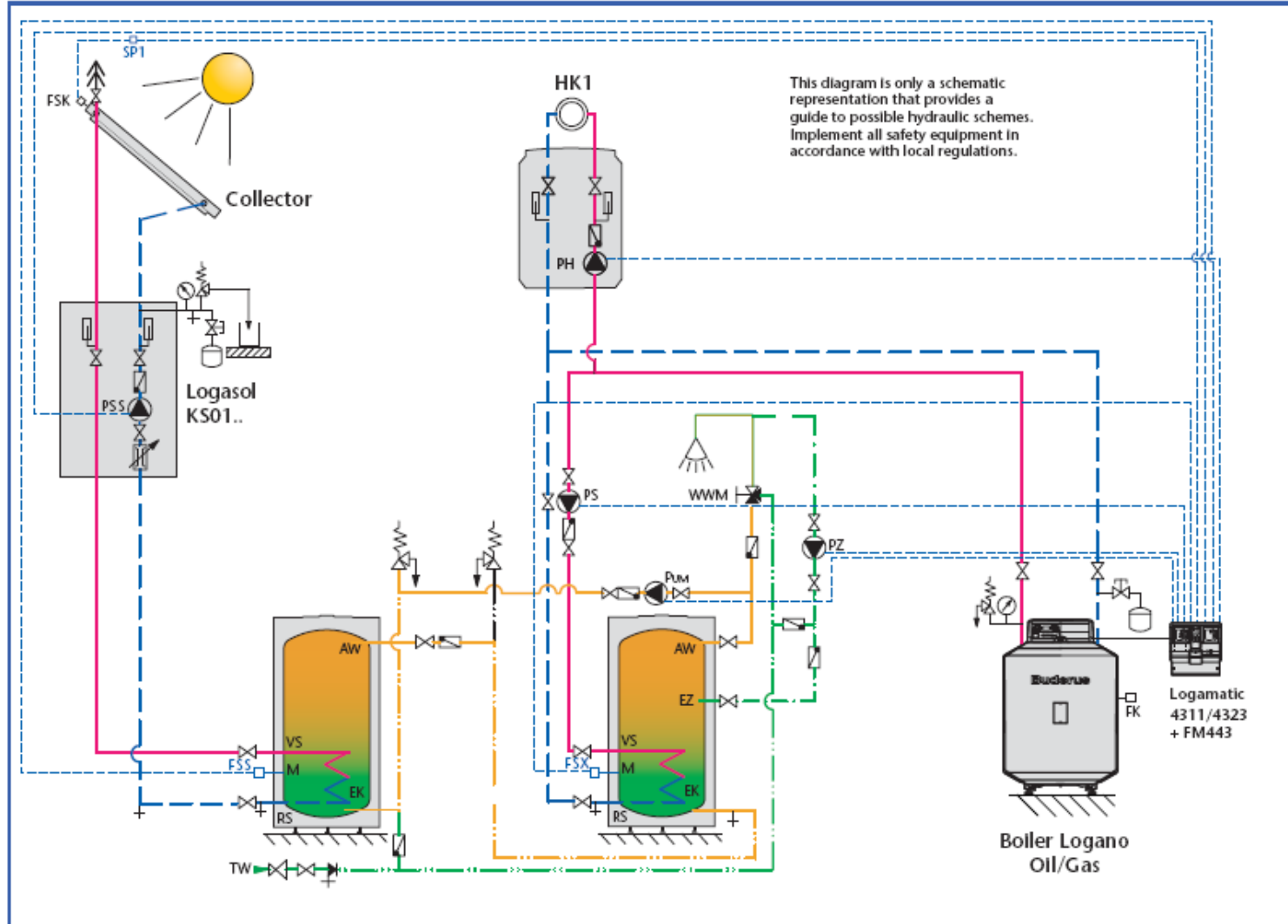
50/1 Diagram of a two-storage tank system with pre-heat storage tank and standby storage tank filled with DHW; storage tank water transfer and disinfection by solar function module FM443
